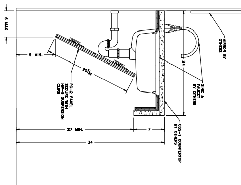
3 VERTICAL SECTION SCALE: 1/2"=1' REF. ARCH. A1/-1-00
