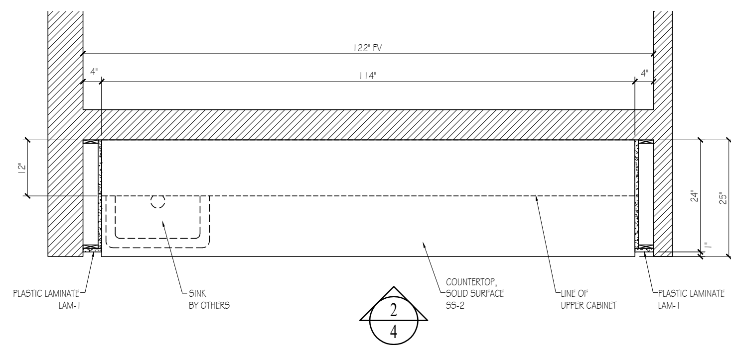
1 PLAN VIEW Scale: 3/4" = 1'-0" COFFEE BAR #107 Arch Ref: 1/A101
