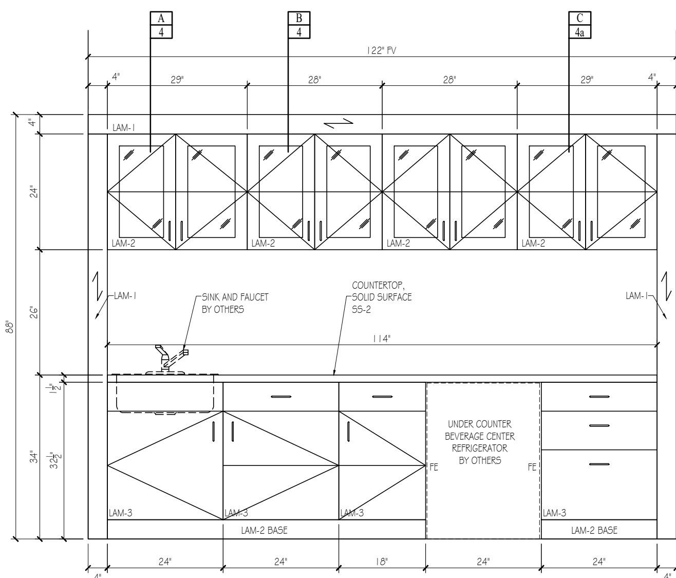
2 ELEVATION Scale: 3/4" = 1'-0" COFFEE BAR #107 Arch Ref: 20/A503
