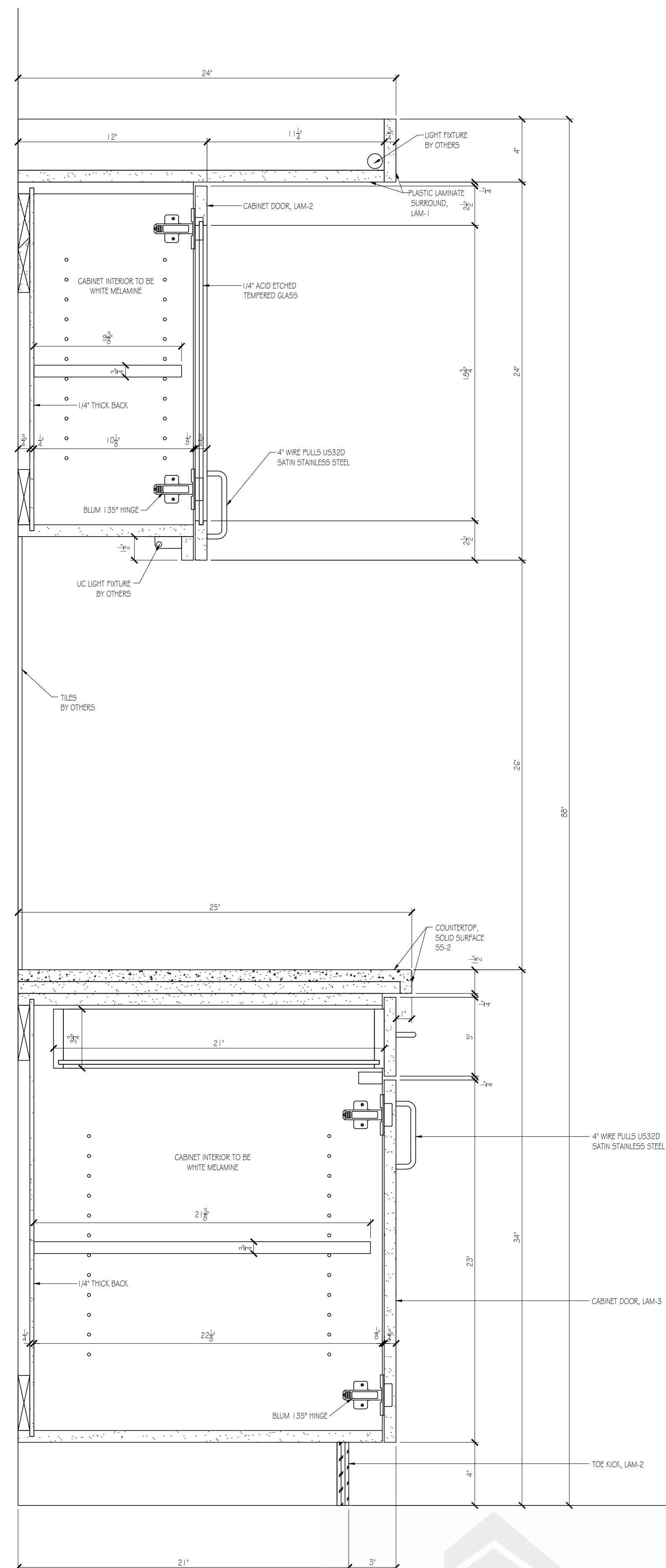
B VERTICAL SECTION @ Cabinet Scale: 3" = 1'-0" Arch Ref: NONE
