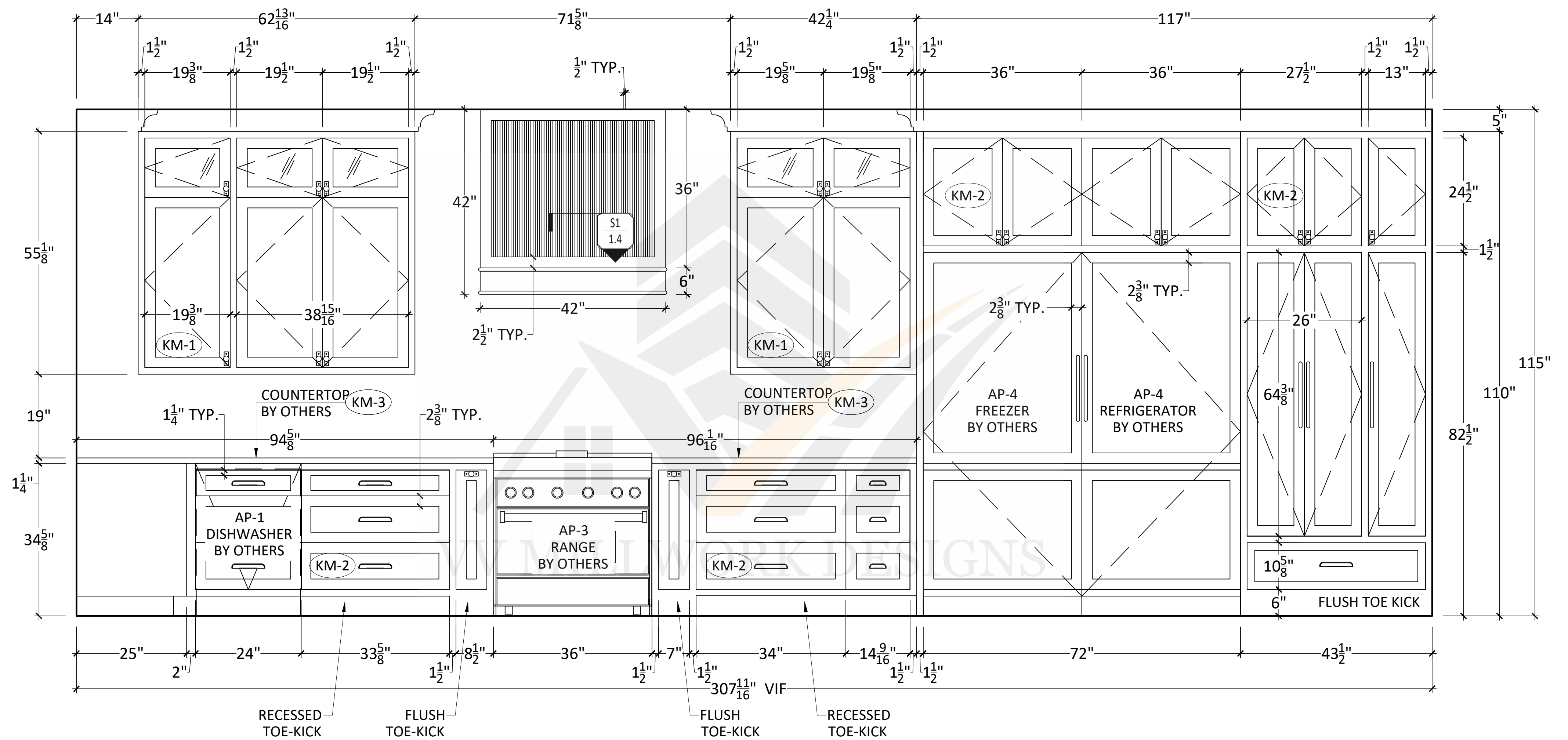
C ELEVATION @ KITCHEN 1.3 NONE 1" = 1'-0"
